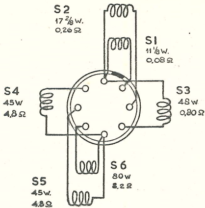
ANTENNE SP. GK 563 51
